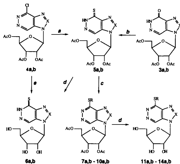
Scheme 1. In series a, X=N; in series b, X=CH. Reagents: (a) Na 2 S 2 O 5 , BuOH, H 2 O, EtOH; (b) P 2 S 5 (series a: S 8 , dioxane; series b: pyridine); (c) NaH, alkyl halide, THF; (d) MeOH/NH 3 ; (e) NaSH, MeOH (series a only).
